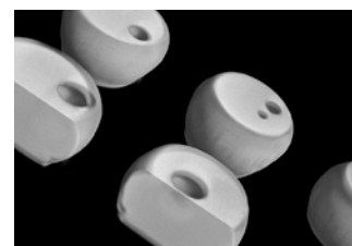
Voids in BGA (CT image)
